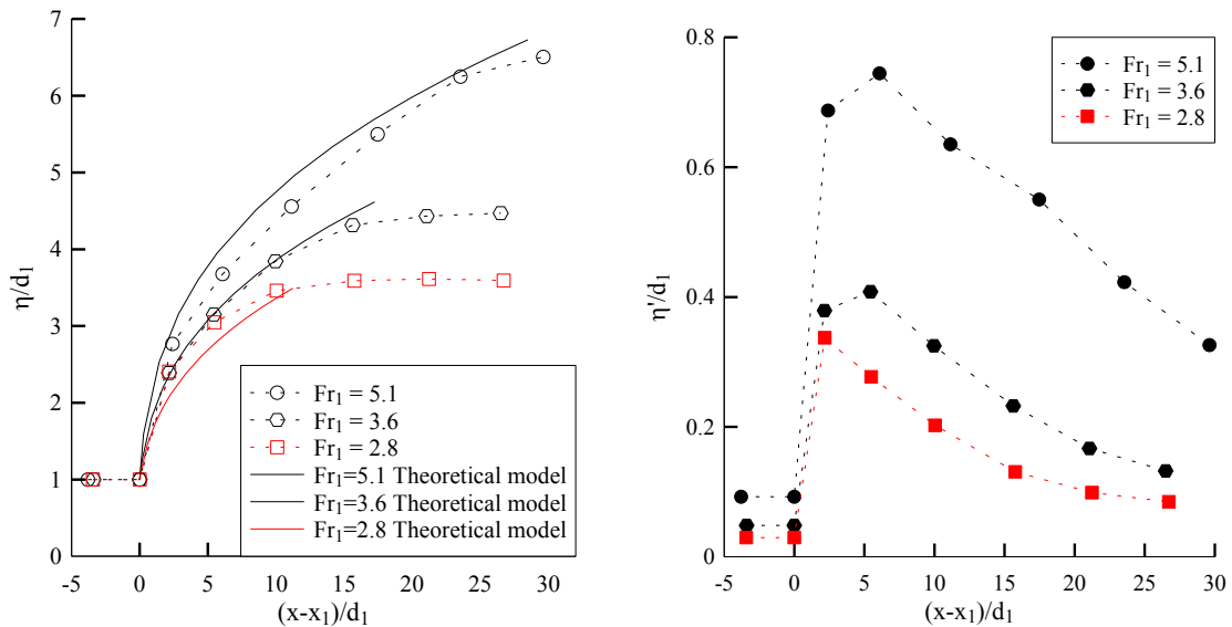
Figure 3 - Longitudinal distributions of dimensionless time-averaged free surface profile \eta/d_1 (Left) and standard deviation of the free surface elevations \eta'/d_1 (Right) - Comparison with the roller surface model of CASTRO-ORGUAZ and HAGER (2010)
