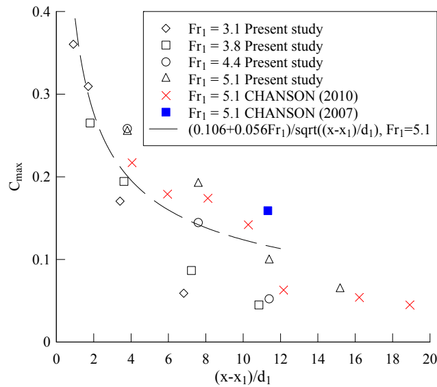
(A) Maximum void fraction C_{\max} in the air-water shear layer
