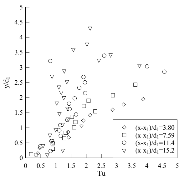
Figure 8 - Dimensionless distributions of streamwise turbulence intensity Tu in hydraulic jump rollers - Fr_1 = 5.1 , Re = 1.3 \times 10^5 , d_1 = 0.0395 m, x_1 = 1.50 m
