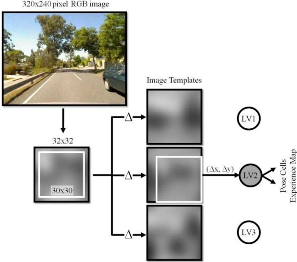
Figure 3 – Visual templates illustration. The resolution reduced current frame is compared against a library of image templates. If a template is matched, it activates the corresponding local view cell, otherwise a new visual template is learned.
