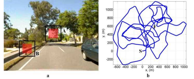
Figure 2 – Visual odometry illustration. (a) Patch locations and search ranges. (b) Trajectory for dataset 1 calculated using the visual odometry system.
