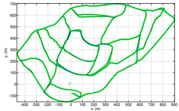
Figure 16 – Experience map for combined dataset 1 and dataset 2, containing 3893 experiences and 4850 inter-experience links, T_D = 0.045 , P = 97.0\% , R = 78.7\% .
