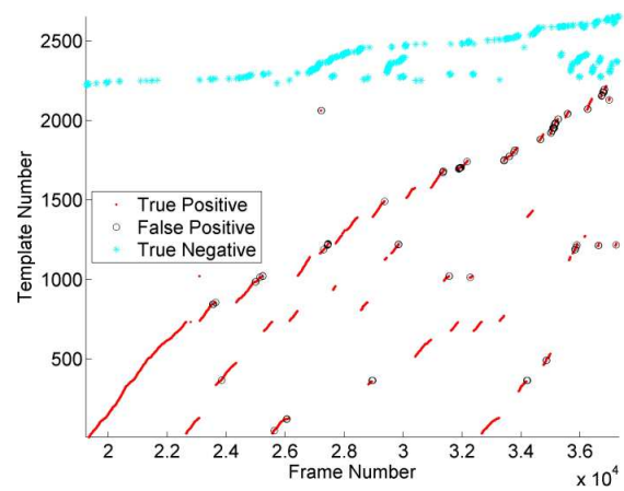
Figure 15 – Template graph for dataset 2 with visual expectation, T_D = 0.045 , P = 97.0\% , R = 78.7\% .
