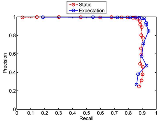
Figure 7 – Precision-recall graph with and without visual expectation for dataset 1. The lines between graph points indicate the direction of increasing default template recognition threshold, T_D .
