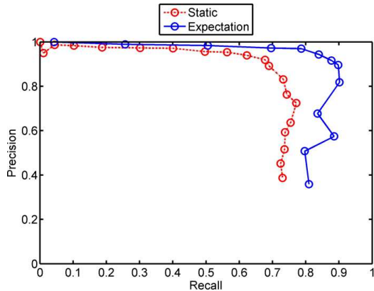
Figure 11 – Precision-recall graph for dataset 2 after processing of dataset 1, with and without visual expectation enabled.
