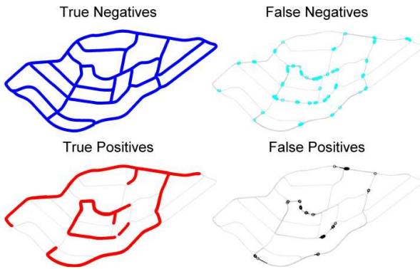
Figure 8 – Ground truth maps with true/false positive/negative classifications superimposed on the robot’s trajectory for dataset 1, with visual expectation enabled. T_D = 0.045 , P = 98.5\% , R = 91.6\% .
