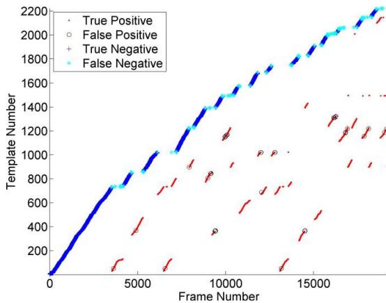
Figure 9 – Template graph for dataset 1 with visual expectation enabled, T_D = 0.045 , P = 98.5\% , R = 91.6\% .
