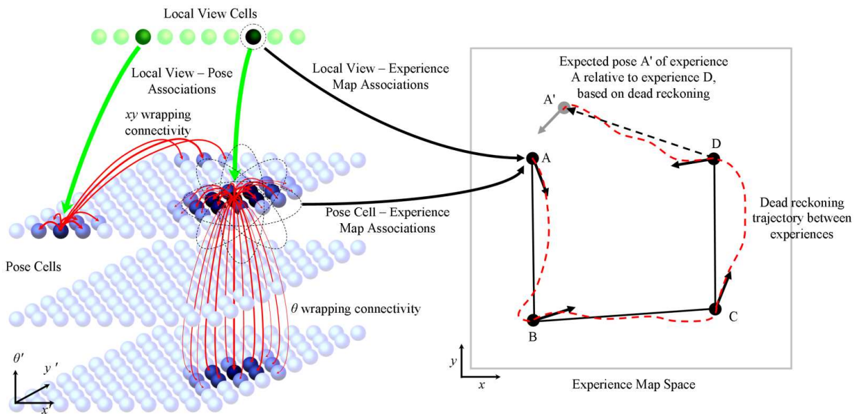
Figure 1 – The RatSLAM pose cell network and experience map. Self-motion and visual data drive activity in the pose cell network, which in turn drives the creation of nodes and links in the experience map.
