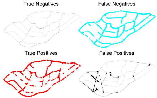
Figure 14 – Frame classifications superimposed on the GPS trajectory without visual expectation, T_D = 0.055 , R = 40.0\% , P = 97.1\% .
