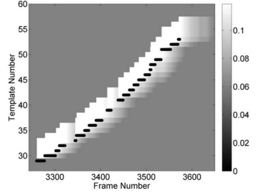
Figure 4 – Enhanced template recognition thresholds due to visual expectation. Dots indicate the currently matched template. The shading level indicates the threshold for visual template comparisons, below which two visual templates are considered to be the same. The lighter shaded areas above each matched template indicate the elevated recognition thresholds for templates immediately following a matched template. The elevated thresholds then decay over subsequent frames.
