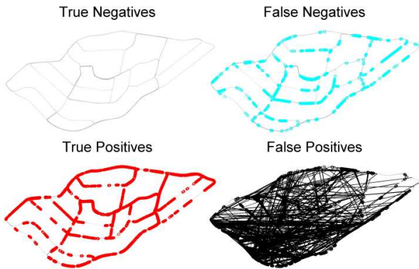
Figure 13 – Frame classifications superimposed on the GPS trajectory without visual expectation, T_D = 0.095 , P = 72.5\% , R = 77.2\% .
