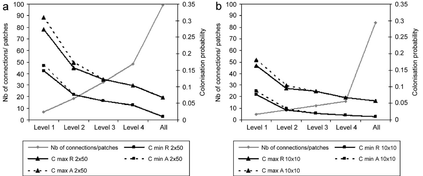
Fig. 3. Minimum and maximum value of colonization rates necessary for metapopulation persistence at different levels of connectivity, with two spatial configurations, (a) 2 \times 50 , and (b) 10 \times 10 , when disturbance is either aggregated ( A ) or randomized ( R ). The left abscissas and the solid squares lines show the number of connections per patch for each level of connectivity, representing the maximum distance between patches for which colonization is possible. The right abscissas and remaining lines indicate the minimum colonization rate for which metapopulations persist (square) and maximum rate for which extinctions occur (triangle) for each level of connectivity and for random (solid line) and aggregate (dashed line) disturbances.
