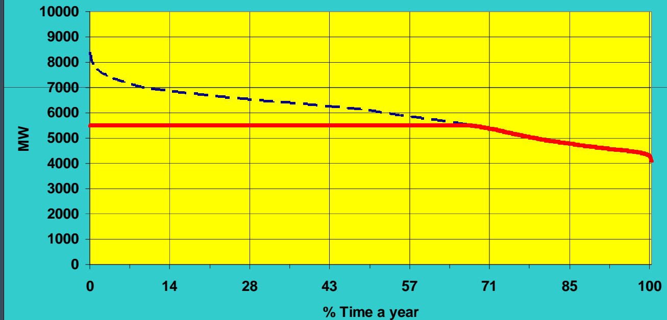
Figure 7 Electricity demand curtailed in Queensland not to exceed $55/MW.
