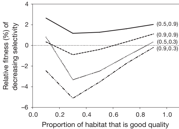
Fig. 2. Relative fitness (% of constant selectivity) of the decreasing selectivity phenotype in environments that vary in the proportion of good quality habitat; 4 combinations of habitat availability ( E_h ) and energy expenditure rates ( \Delta x ) are shown, and parameter values are presented as ( E_h, \Delta x ) such that the top 2 lines represent conditions under which energetic costs of searching are high. Lines above 0% indicate a fitness benefit of decreasing selectivity, and those beneath 0% indicate a cost of decreasing selectivity such that constant selectivity would be favoured
