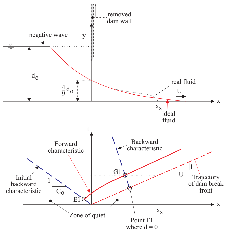
Fig. 17.14 Sketch of dam break wave in a dry horizontal channel (CHANSON 2004, The hydraulics of open channel flow: a introduction, Butterworth-Heinemann, 2nd edition)
