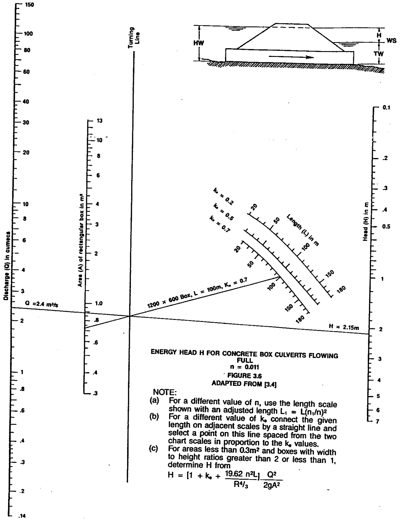
Fig. IV-4-6 - Hydraulic calculations of total head losses for concrete box culverts flowing full (i.e. drowned) (Concrete Pipe Association of Australasia 1991, p. 41)
